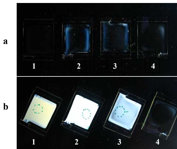
Figure 1. The cells filled with RM UCL-011 viewed between a pair of crossed polarizers: (a) the in-plane projection of optical axis is parallel to the polarization of incident light; (b) the in-plane projection of optical axis is tilted to the polarization of incidence light. The tilt angle of optic axis is 3^\circ , 33^\circ , 56^\circ and 89^\circ in cells 1, 2, 3 and 4.
