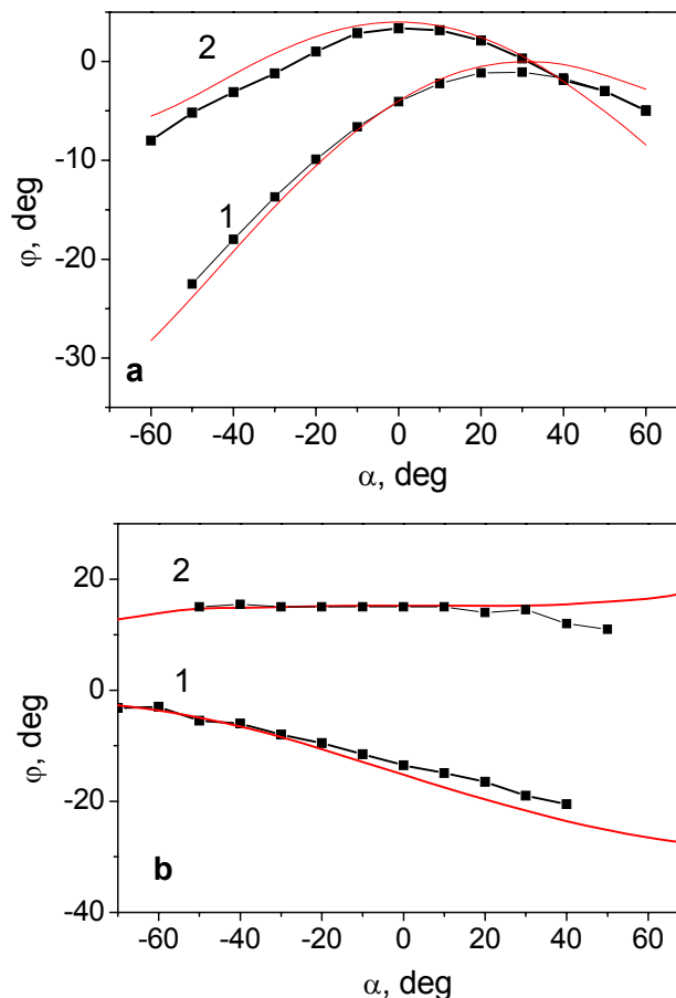
Figure 4. Measured (dots) and modeled (solid lines) analyser vs. light incidence angle curves for cells 1 (a) and 2 (b) presented in Fig. 3. The curves 1 and 2 correspond to two measuring positions of the cell, when in-plane projection of optic axis is orientated horizontally and vertically, respectively.
