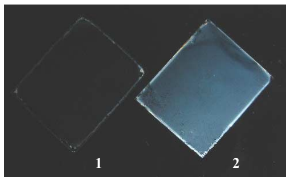
Figure 3. The films of UCL-011 (1) and UCL-017 (2) coated over rubbed p-PI/h-PI (4:1) layers viewed between a pair of crossed polarizers. The in-plane projection of optical axis is tilted to the polarization of incidence light.
