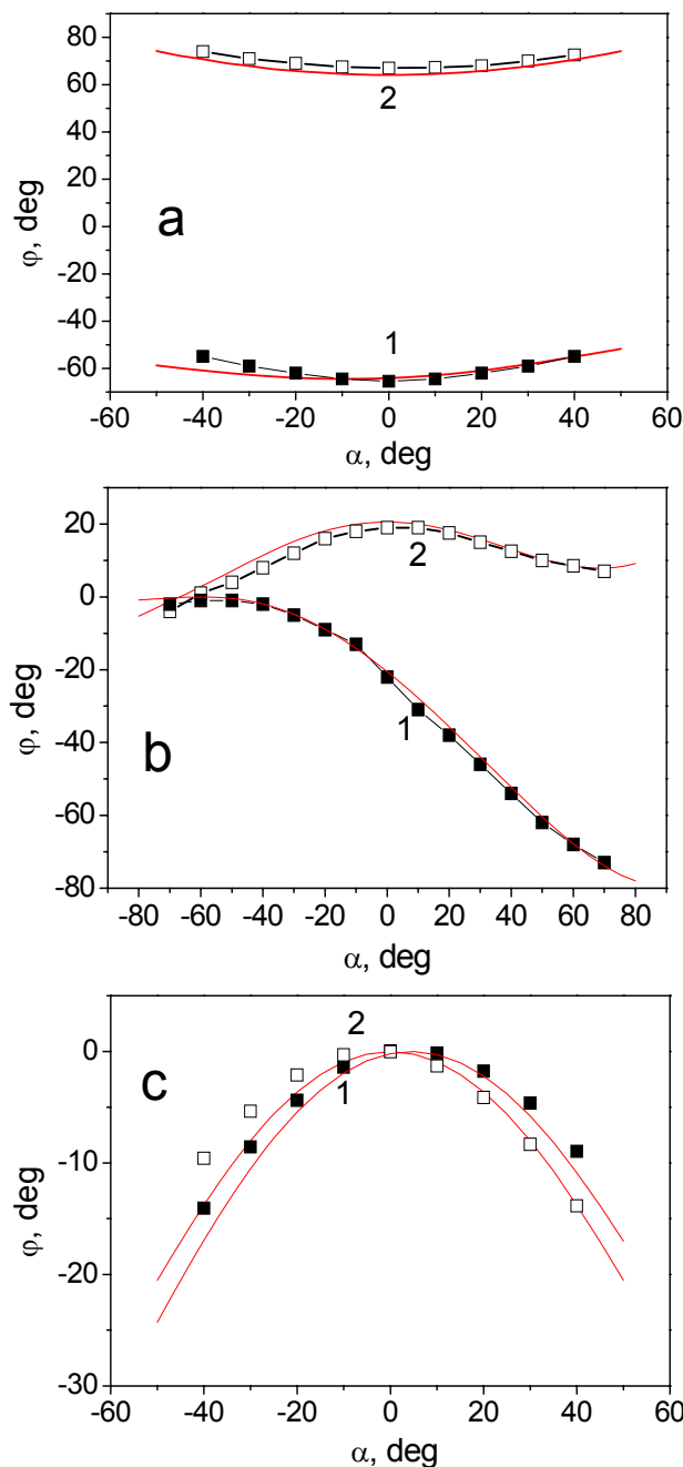
Figure 2. Measured (dots) and modeled (solid lines) analyser vs. light incidence angle curves for cells 1 (a), 2 (b) and 4 (c) from Fig. 1. The curves 1 and 2 correspond to two measuring positions of the cell, when in-plane projection of optic axis is orientated horizontally and vertically, respectively.
