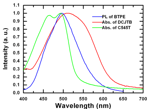
Figure 2. PL spectrum of BTPE as well as absorption spectrum of DCJTb and C545T.
